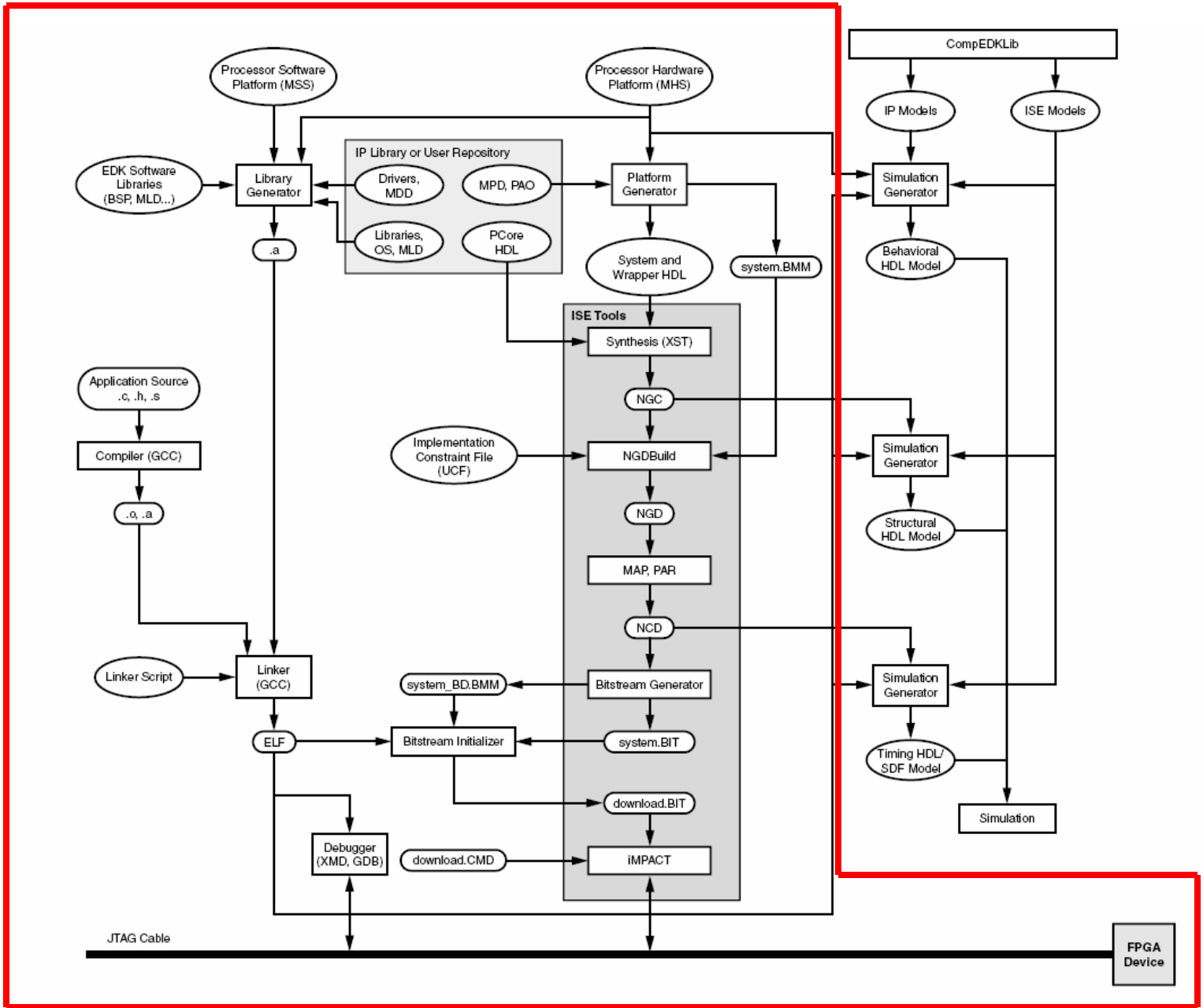
Drawing of the Embedded Development Kit (EDK) Tools Architecture
